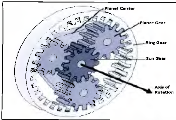
Figure 4: illustrates the components of planetary-gear set (Wendelius, 2012)
