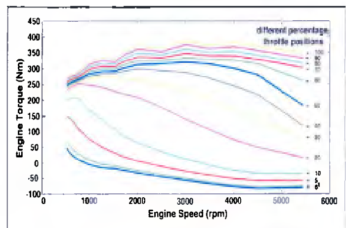
Figure 19: Engine Torque map data used in simulation
