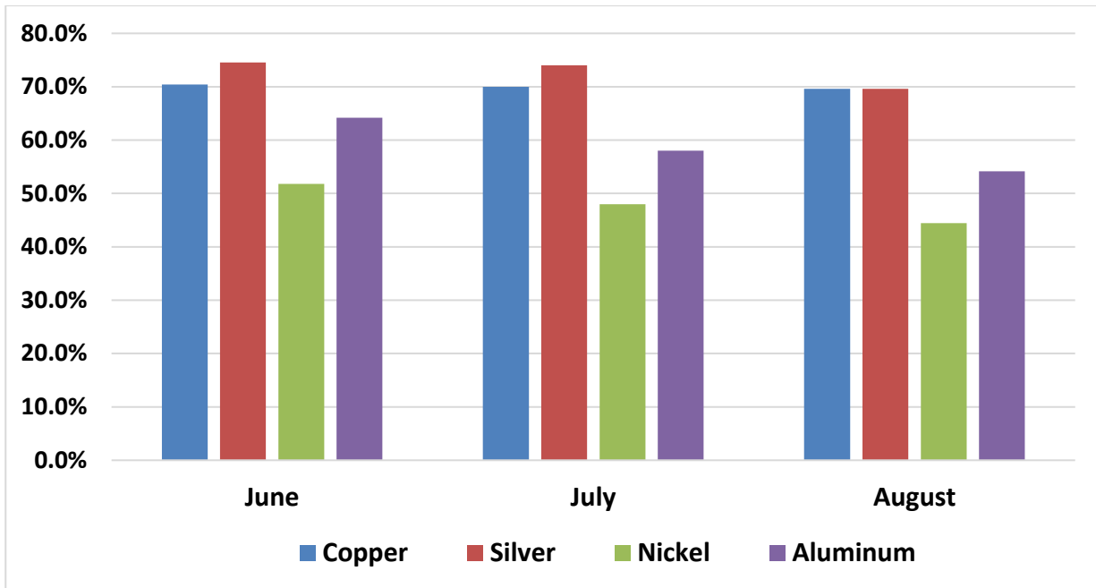
Figure 3.4. Efficiency Comparison for 4 absorber materials at summer months
