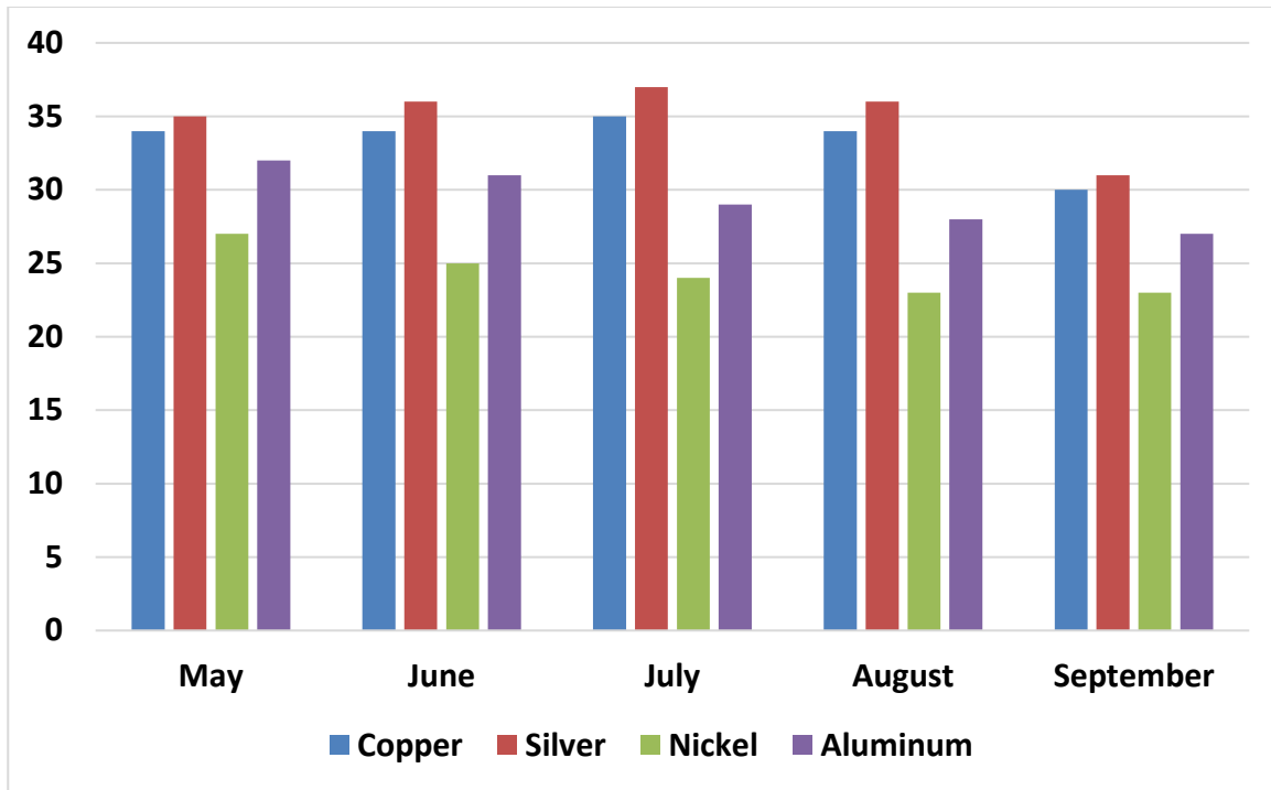
Figure 3.2. Temperature Difference comparison in May, June, July and Sept. months for 4 absorber material
