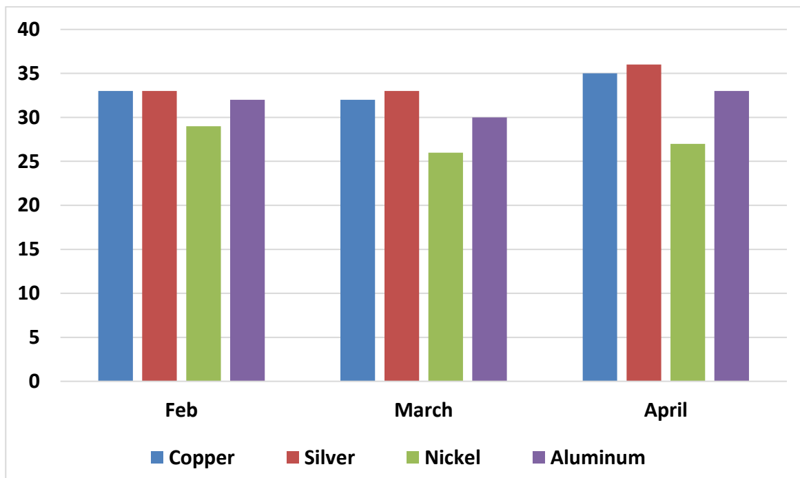
Figure 3.1. Temperature Difference comparison in Feb, March, and April months for 4 absorber material
