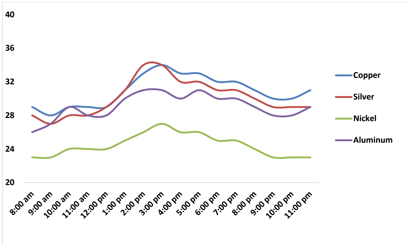
Figure 3.3. Temperature Difference along one day for 4 absorber material
