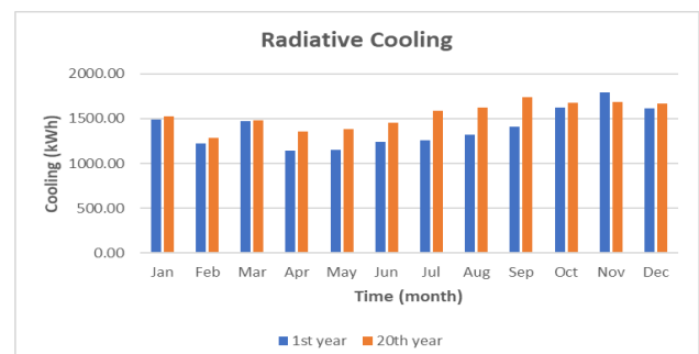
Figure 7: Solar cooling gain for each month in the first and 20th year of simulation.
